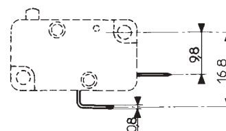
W3 for 6.35 mm push-on
